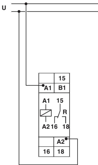
Figure 2 Switched-mode beginning with pause
