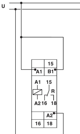
Figure 3 Switched-mode beginning with pulse
